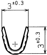
WIRE BARREL
